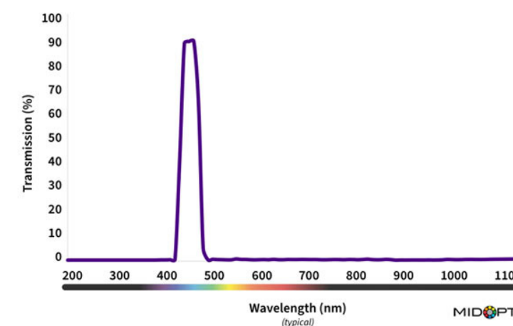
BN450 NARROW INDIGO BANDPASS
